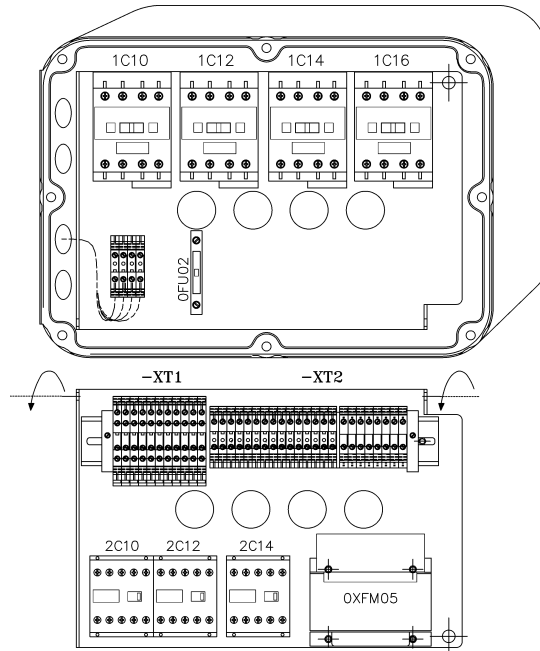
5T and 7½T Electrical Component Positions
