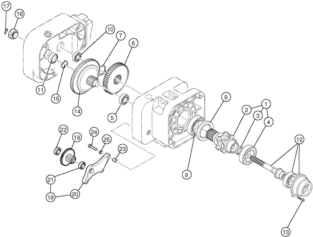
Figure 2-2 Gearing Parts
